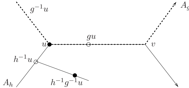
Figure 3: Coherent axes
