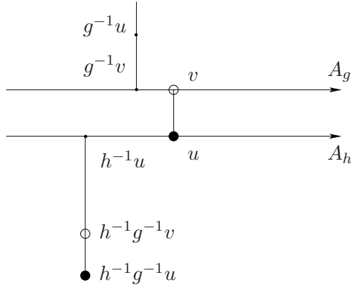
Figure 2: Disjoint axes
